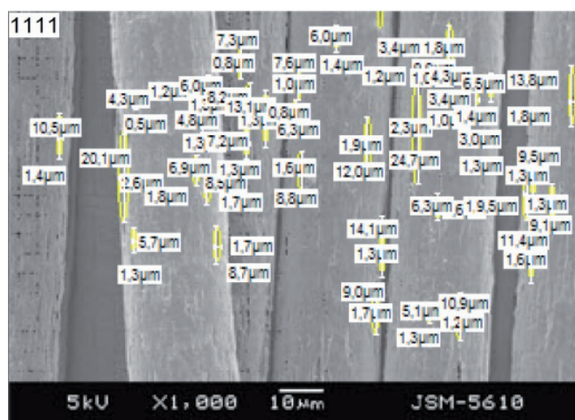
Figure 2. Measured pore sizes by JEOL SMile View software.
