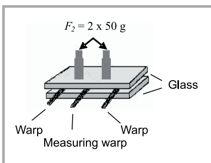
Figure 4. Warp yarn measurement under loads.
