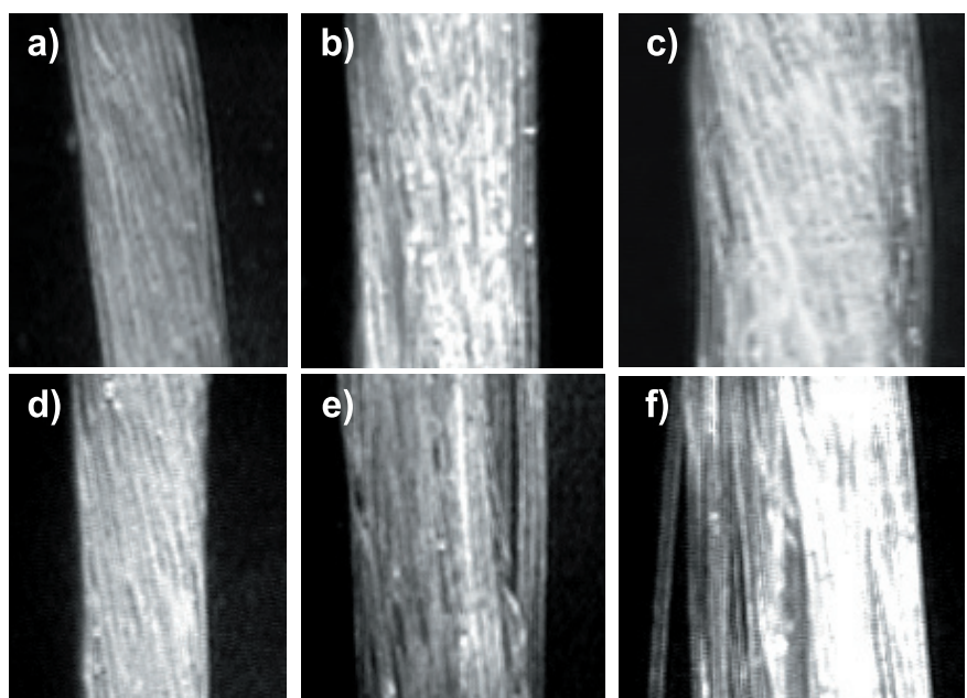
Figure 5. Warp projections under 10 g load: a) l=0 cm, b) l=1 cm, c) l=2 cm and warp projections under 60 g load: d) l=0 cm, e) l=1 cm, f) l=2 cm.
