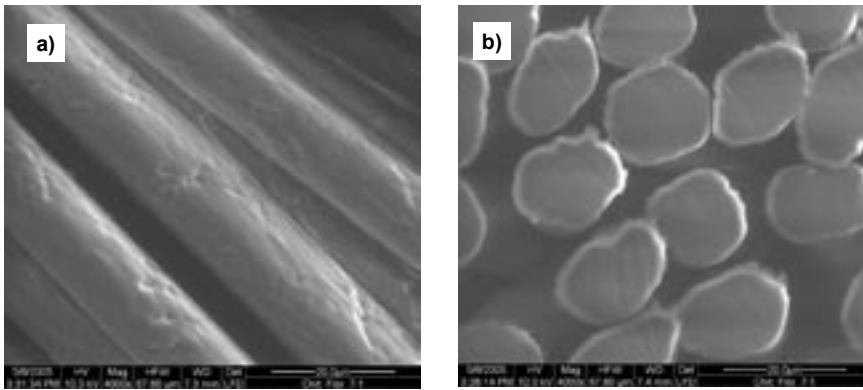
Figure 3. Photos from the scanning electron microscope (SEM) of the chitosan/silk-fibroin fibres Ch/SF III with a silk-fibroin content of 11 %; a) view of the fibres' surfaces, b) view of the fibres' cross-sections.
