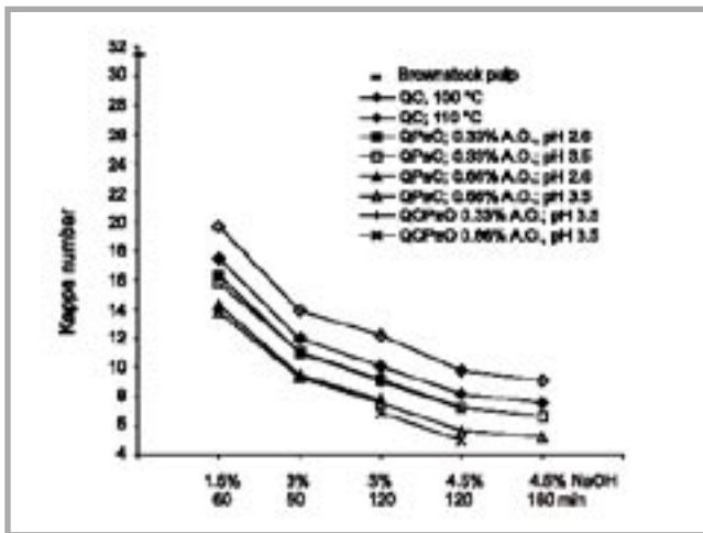
Figure 1. Kappa number values obtained in different variants of the oxygen delignification of pine kraft pulp, kappa number 31.5. (Standard deviation of kappa number determination was 0.1).
