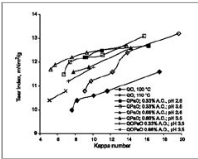
Figure 3. Relationship between tear index and kappa number of oxygen-delignified pine kraft kappa number 31.5 pulp in different variants of the process. (Standard deviation of tear index measurements was 0.2 \text{ mN} \cdot \text{m}^2/\text{g} ).
