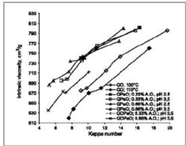
Figure 4. Relationship between kappa number and intrinsic viscosity of oxygen-delignified pine kraft kappa number 31.5 pulp in different variants of the process. (Standard deviation of viscosity was 8 \text{ cm}^3/\text{g} ).
