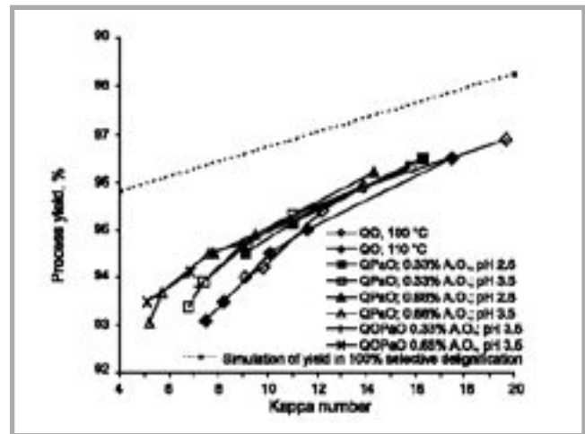
Figure 2. Yield-to-kappa number relationship in different variants of oxygen delignification of pine kraft pulp, kappa number 31.5. (Standard deviation of yield amounted to 0.14%).
