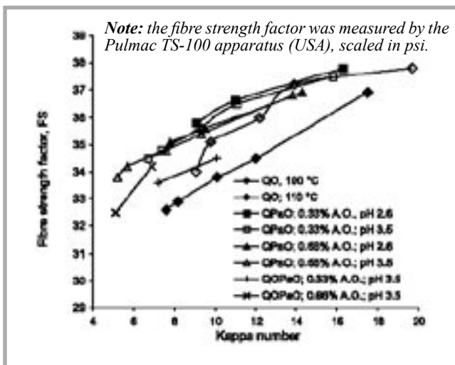
Figure 5. Relationship between zero-span fibre strength factor and kappa number of oxygen-delignified pine kraft kappa number 31.5 pulp in different variants of the process (after beating the pulp in a Jokro mill to freeness 20^\circ\text{SR} , beating time 12 min.); (Standard deviation of FS-factor was 1.1).
