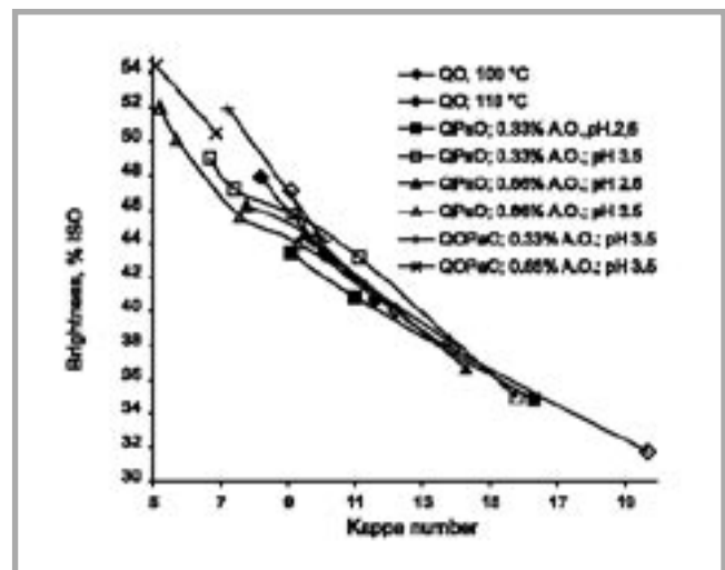
Figure 6. Relationship between kappa number and ISO brightness in different variants of oxygen delignification pine kraft pulp, kappa number 31.5. (Standard deviation of ISO brightness was 0.2%).
