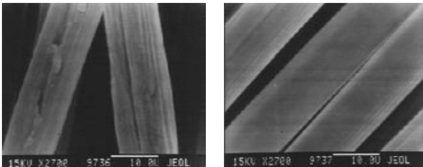
Figure 5. SEM photographs of AW fibres; a) – untreated, b) – modified by cellulase Eiconase CE.
