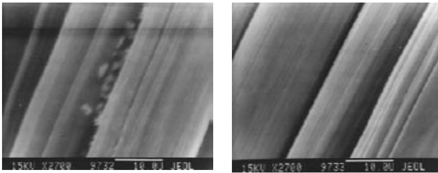
Figure 4. SEM photographs of Celsol fibres; a) – untreated, b) – modified by cellulase Eiconase CE.
